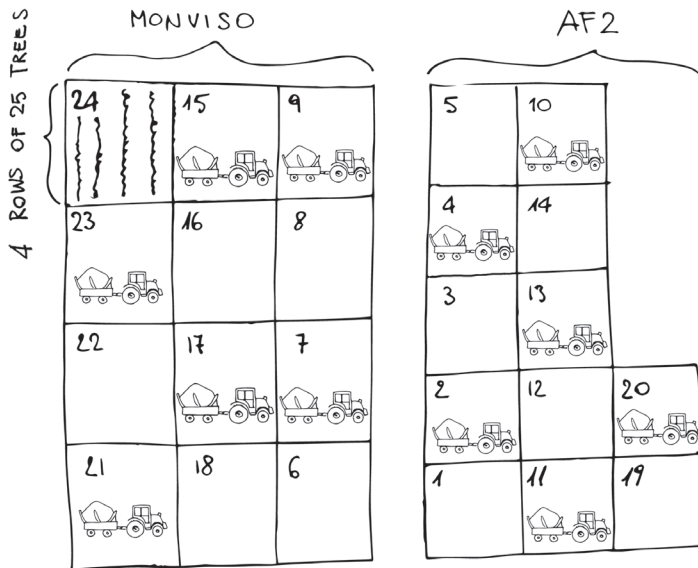
Figure 3 – Design of an experiment for comparing terrain chipping vs. roadside chipping in a short-rotation poplar plantation. Plots are allocated randomly to the two treatment levels (i.e. terrain chipping = blank plots; roadside chipping = plots with a forwarder symbol). The experiment is blocked for two main clone types, i.e. Monviso and AF2. It is therefore a factorial 2 x 2 design, where each of the 4 treatments is repeated 6 times (i.e. total of 24 replications). Hence the design is balanced.
